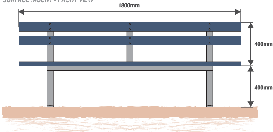
SURFACE MOUNT - FRONT VIEW
