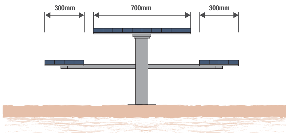
END VIEW
