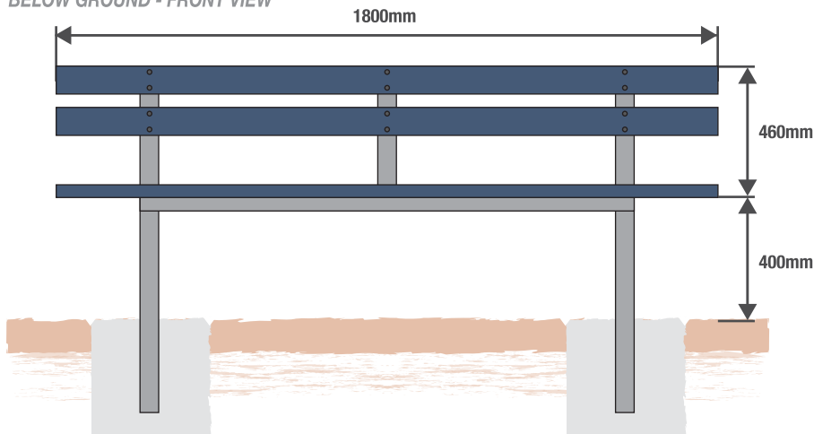
BELOW GROUND - FRONT VIEW
