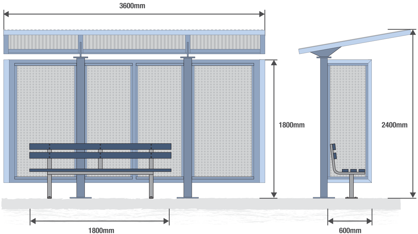
FRONT VIEW
