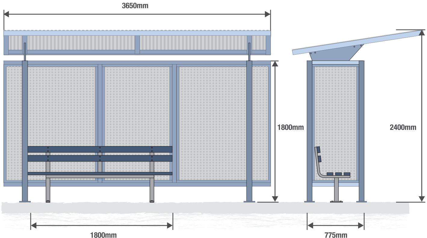
FRONT VIEW
