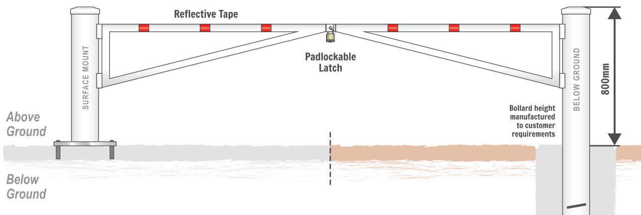
DOUBLE GATE
